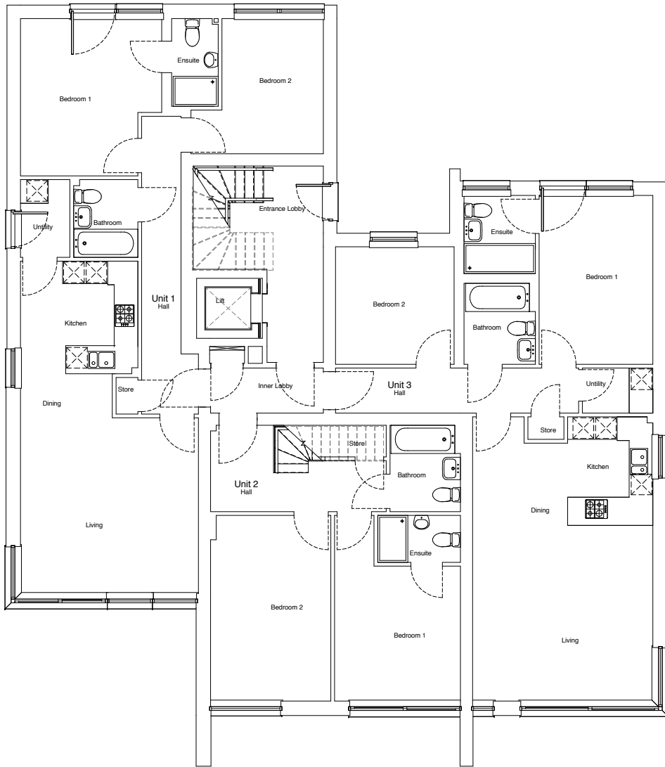
Lower Grd Floor GA 1 : 50
