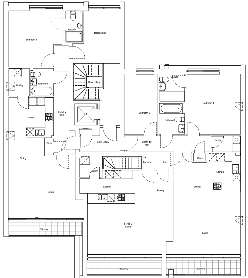
2nd Floor GA 1 : 50
