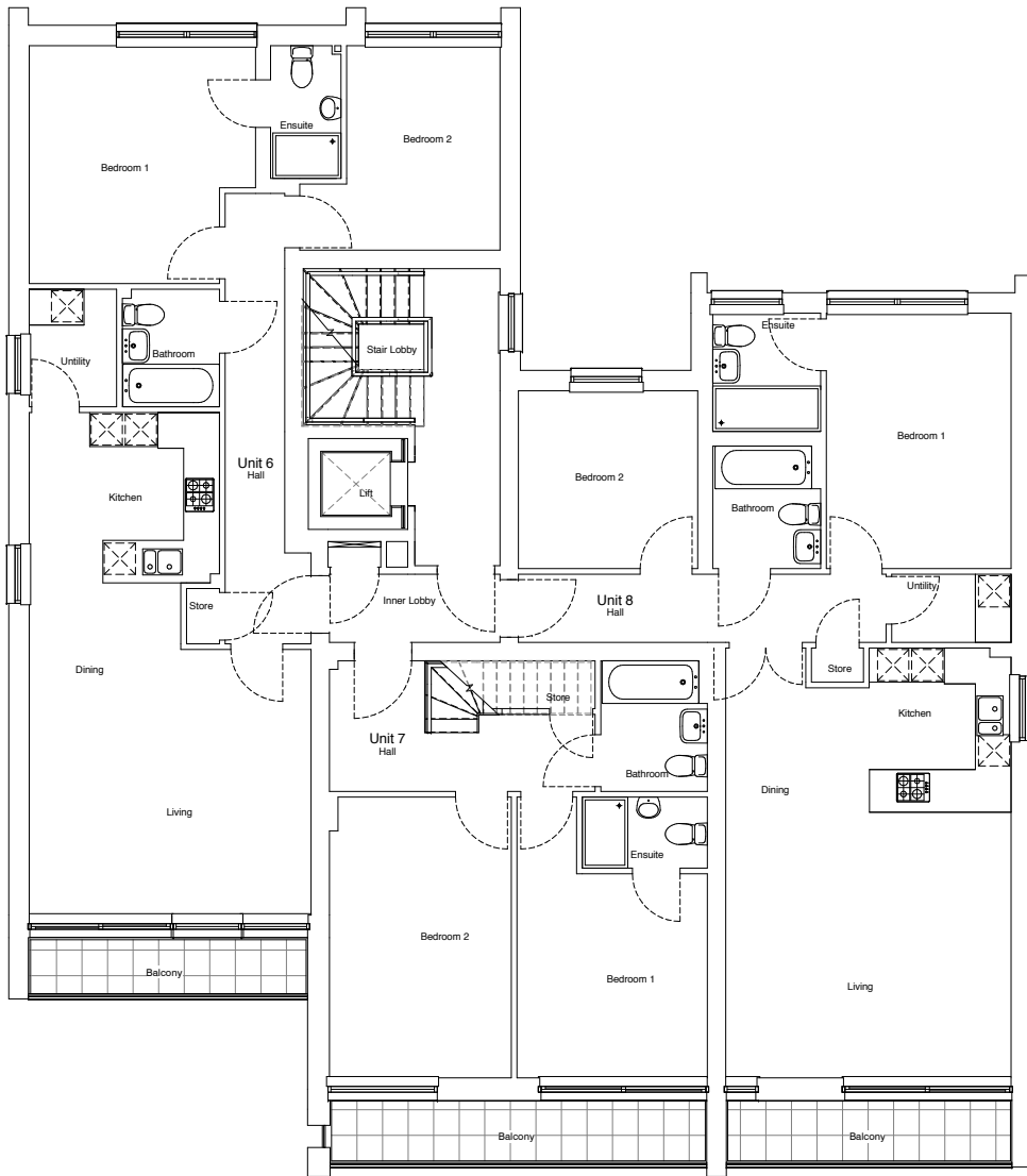
1st Floor GA 1 : 50
