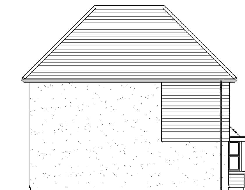
SOUTH-WEST ELEVATION
